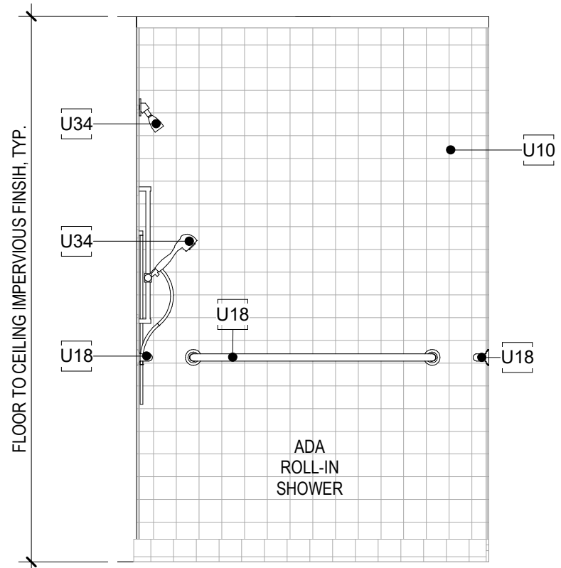
2 UNIT B2 FA MASTER BATH EL. SCALE: 1/2" = 1'-0"
