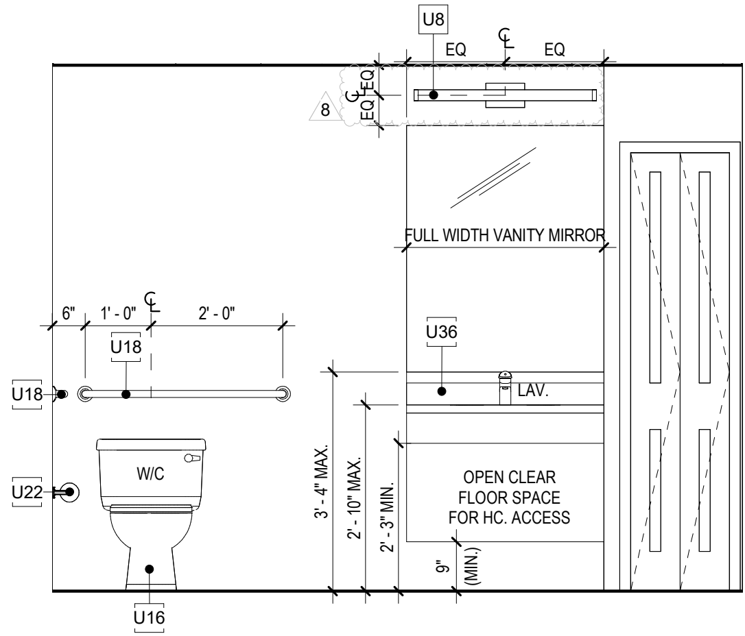
1 UNIT B2 FA MASTER BATH EL. SCALE: 1/2" = 1'-0"
