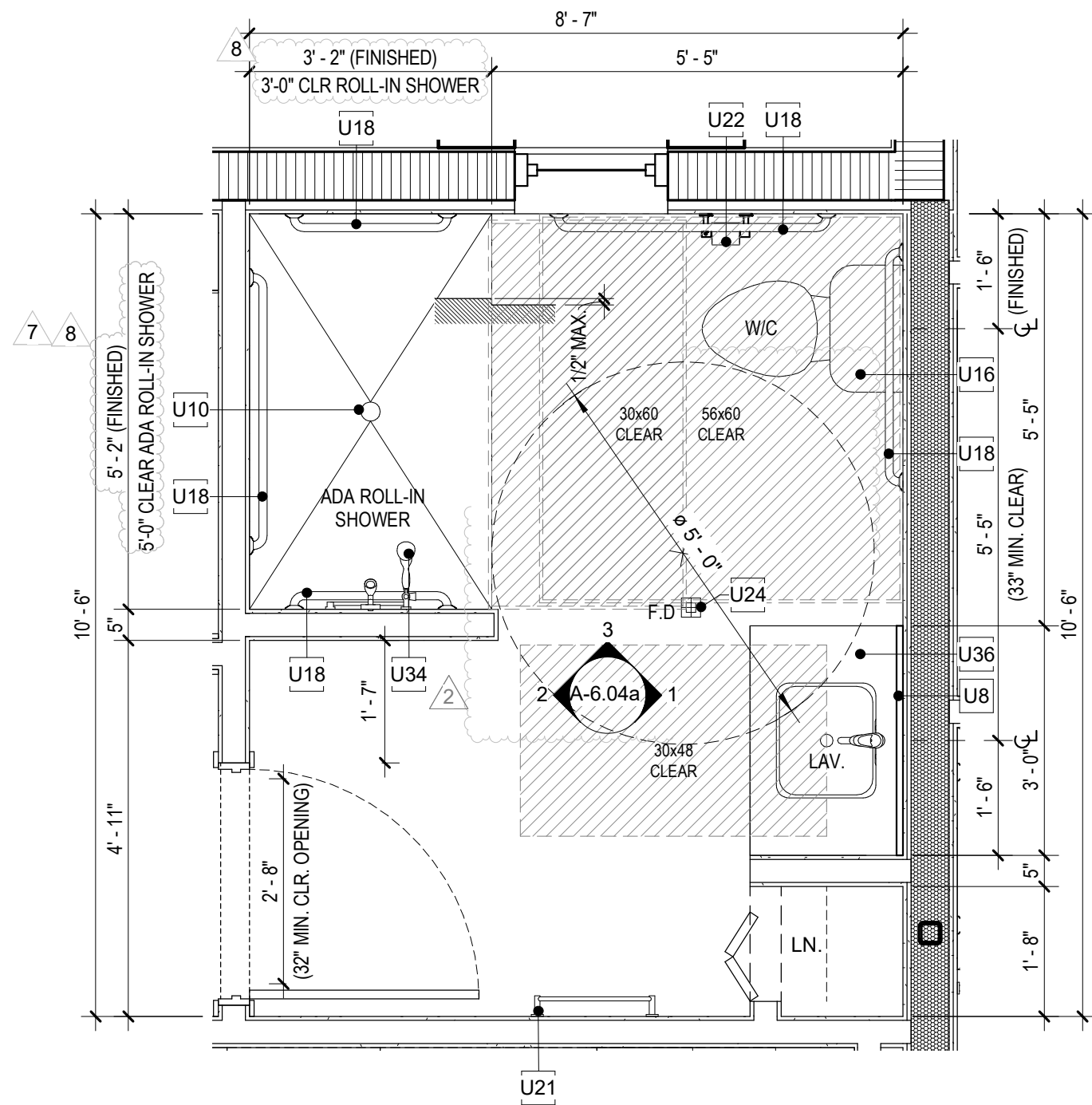
A UNIT B2 FA MASTER BATH PLAN SCALE: 1/2" = 1'-0" TYPE B BATH
