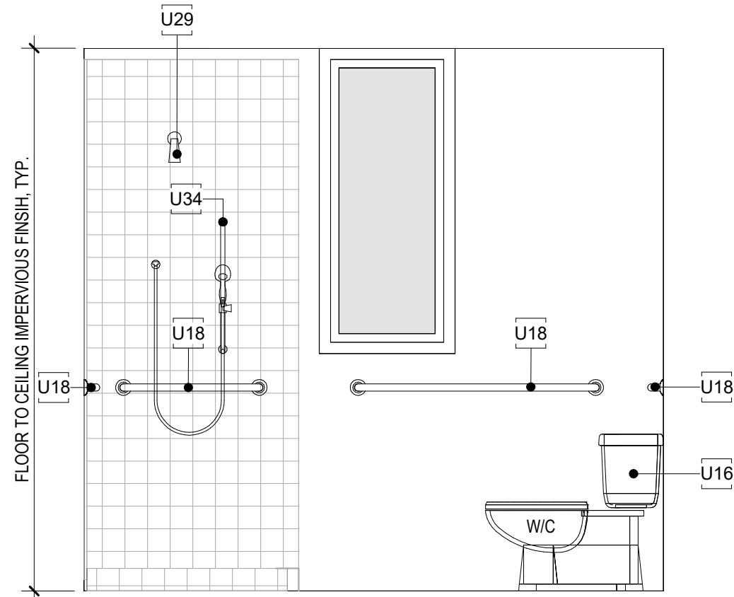
3 UNIT B2 FA MASTER BATH EL. SCALE: 1/2" = 1'-0"
