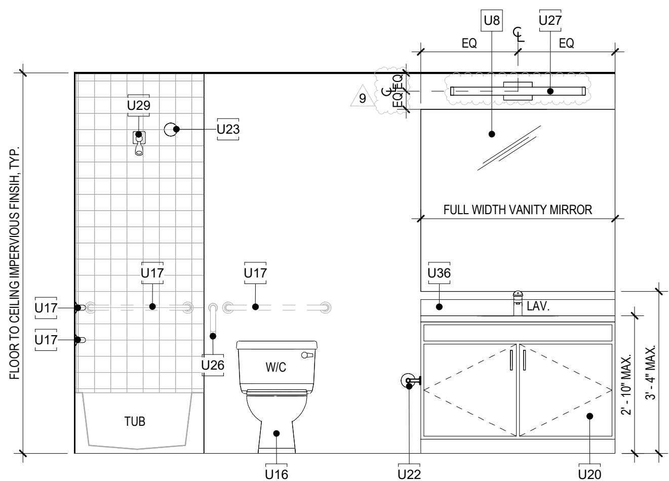
4 UNIT B2 FA BATHROOM EL. SCALE: 1/2" = 1'-0"
