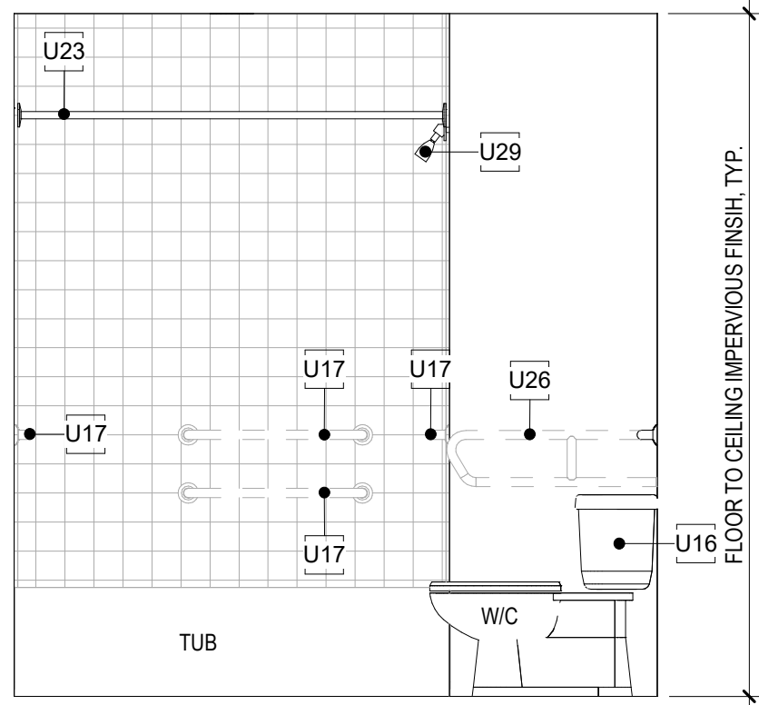
5 UNIT B2 FA BATHROOM EL. SCALE: 1/2" = 1'-0"
