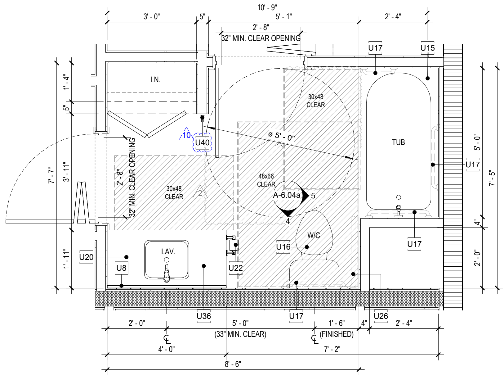
B UNIT B2 FA BATHROOM PLAN SCALE: 1/2" = 1'-0" TYPE B BATH
